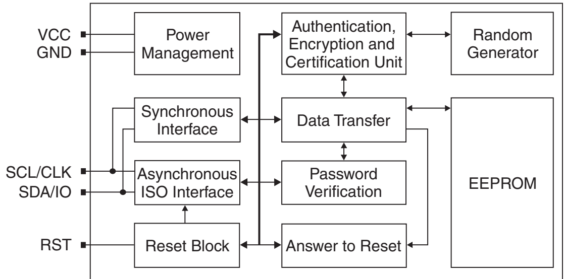
Figure 4-1. Block Diagram
