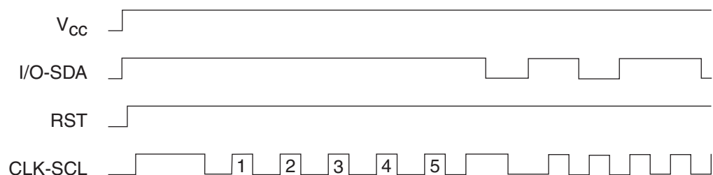
Figure 13-1. Synchronous 2-Wire Protocol
